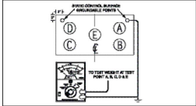
Figure 4. Periodic Performace Tests of Installed Surfaces.
